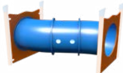
Zig-Zag Crawl Tunnel Left or Right Zig-Zag Ages: 2-5, 5-12 Decks: Equal Height Offset by 24" Available for 5" Posts with 48" Decks or 3.5" Posts with 46.5" Decks
