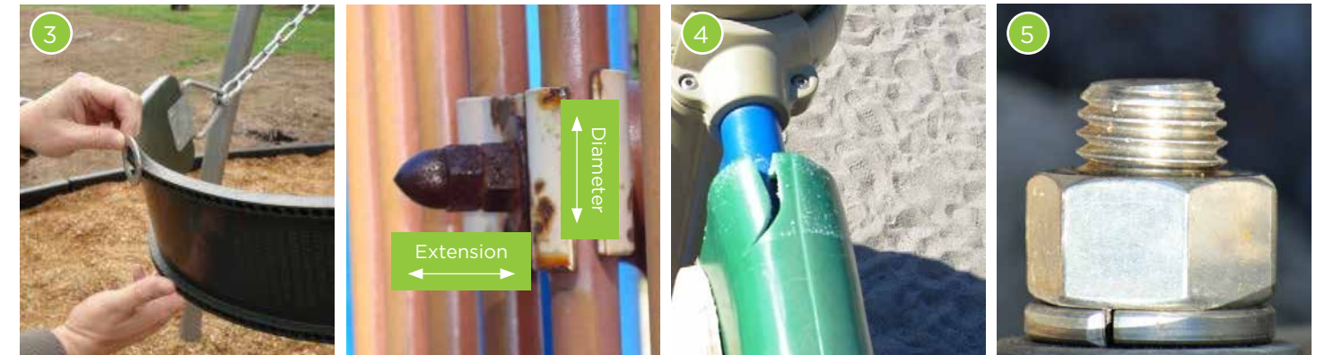
Test swings for protrusion hazards with this special gauge.
