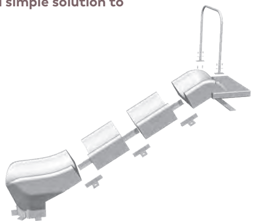
Slide Assembly
